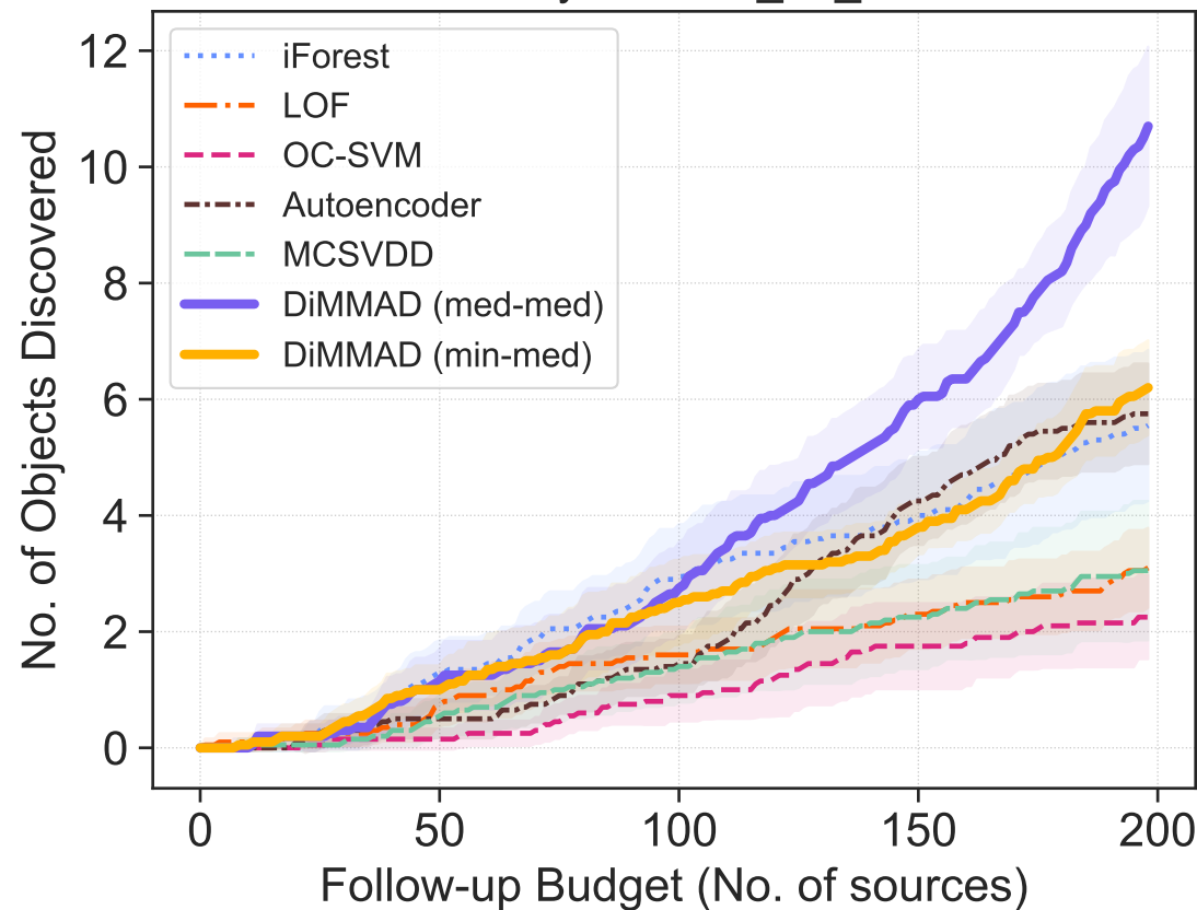
Anomaly: SLSN-I_no_host
